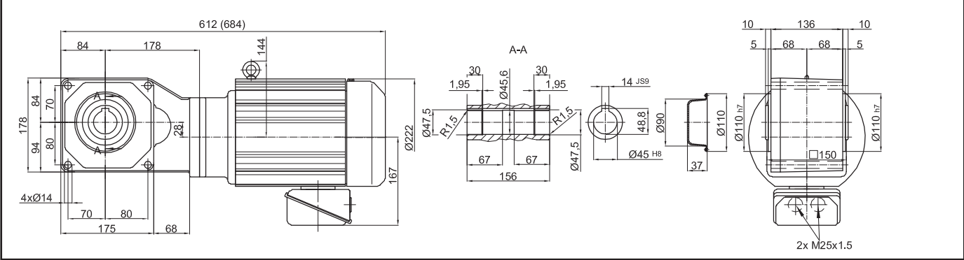
Fig 2 RNYM4-1522E-5 ~ 15 (RNYM4-1522E-B-5 ~ 15) Mass 47 kg (Mass 58 kg)
