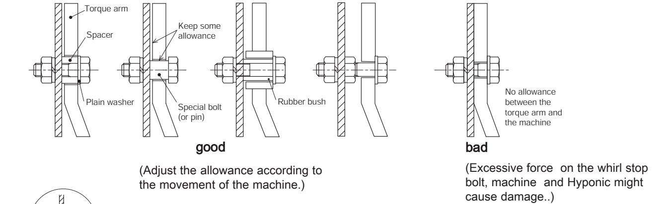
Fig.8 Example of whirl stop mounting (Section A)
