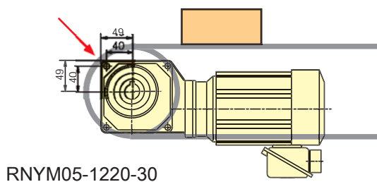
Horizontal mounting
