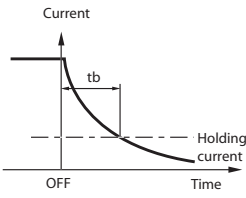
Fig. 3 current curve of standard braking circuit
