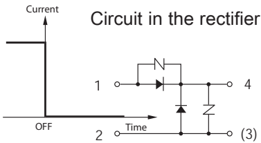
Fig. 4 current curve or quick braking circuit
