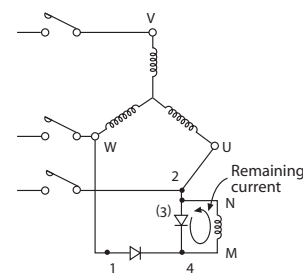
Fig. 1 standard circuit
