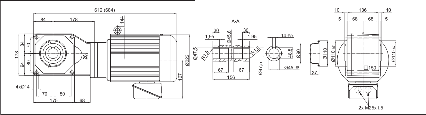
Fig 1 RNYM4-1521E-5 ~ 25 (RNYM4-1521E-B-5 ~ 25) Mass 47 kg (Mass 58 kg)
